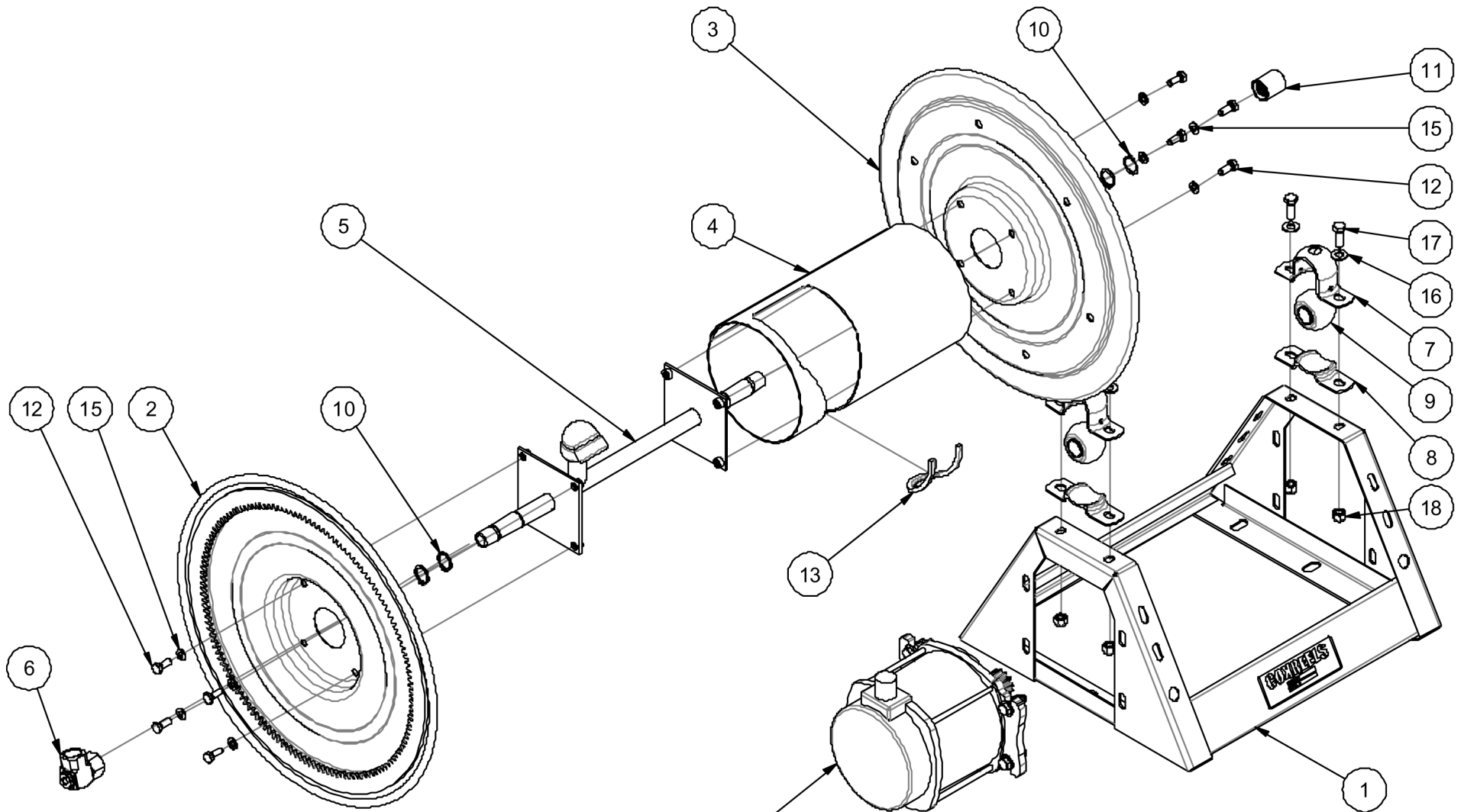
MOTOR OPTIONS AVAILABLE ON 1125 SERIES REELS (FOR INDIVIDUAL PART NUMBERS SEE DRAWING #CM-1125)
